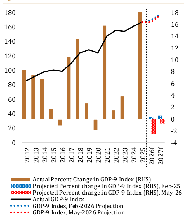
Figure 2: GDP-9 Index
